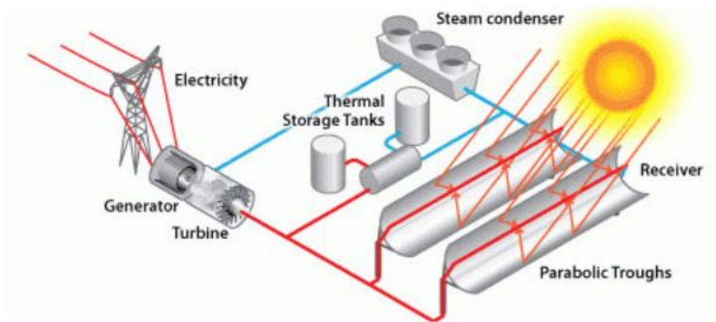
Figure 20: Parabolic through system
