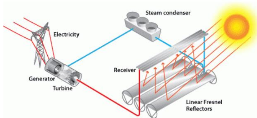
Figure 21: Linear Fresnel Reflector Systems
