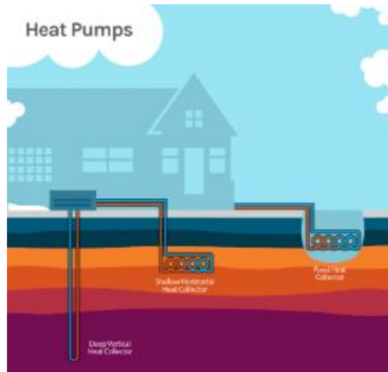
Figure 8: GHP system
