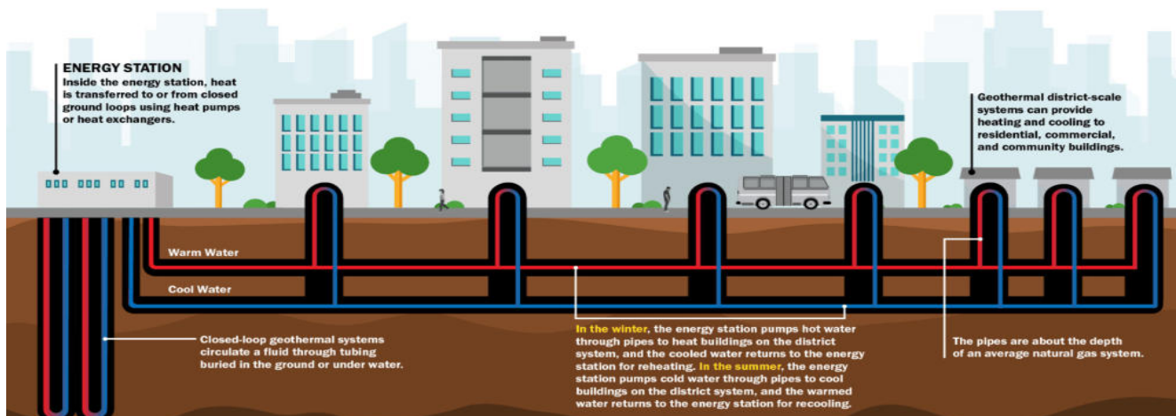
Figure 9: Geothermal District Heating
